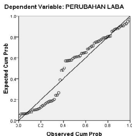
Gambar 3. Normal P-P Plot Regression Standardized Residual
