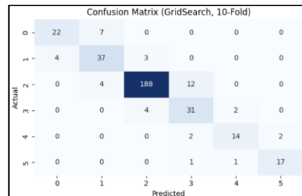
Gambar 10. Confusion matrix uji GS CV 10-fold
