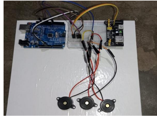
Gambar 16. Buzzer
