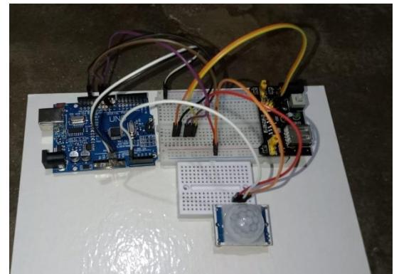
Gambar 17. Sensor PIR
